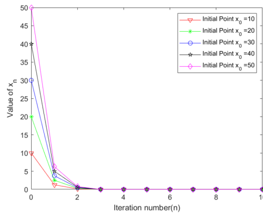
Figure 2 Convergence behavior
